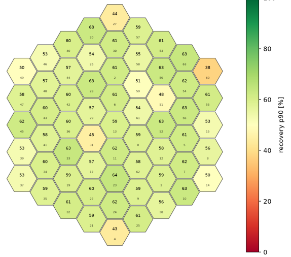
Figure 6: Recovery per channel over the 61 active sensors, at the 90th percentile (left) and on average (right). The colour scale is common to both panels. Recovery degrades towards the perimeter of the array.
