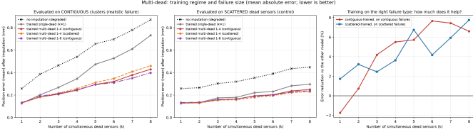
Figure 8: Recovery as a function of the number of simultaneously suppressed channels, for a model trained on single failures and one trained on one to four.
